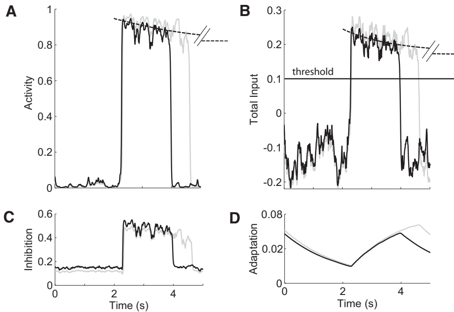
FIG. 4. Dynamical properties of the 2-variable rate-based model. Time courses of dynamical variables of an excitatory neural population in Eqs. B5–B7. The population undergoes transitions between suppressed and dominant states. During dominance, its activity ( A ) and total input ( B ) are lower for strong stimulation ( g_{A,B} = 0.05 , black curves) than for weak stimulation ( g_{A,B} = 0.01 , gray curves). This reduction occurs due to stronger inhibition ( C ). Adaptation current ( D ) is affected by stimulus strength the same way as the activity. Horizontal line in B corresponds to the threshold ( \theta = 0.1 ) of the input–output transfer function of the excitatory neurons (Eq. B5). For the low-stimulation case, the dashed curves are the rate ( A ) and the total input ( B ); they correspond to the attractor’s asymptotic or steady-state values for activity ( A ) and total current ( B ) in the absence of noise and given the instantaneous level of adaptation. Notice that this asymptotic level is well above the transition threshold (horizontal line) of the system. Identical external noise was used for the simulation in the 2 cases.
