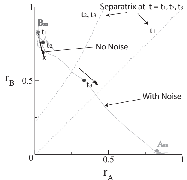
FIG. 5. Adaptation alone, in a noise-free network, does not produce alternations. Smooth trajectory in the (r_A, r_B) phase plane starts from the initial point B_{on} and evolves to a steady-state point, marked by “x”; the trajectory does not reach the separatrix (diagonal line t_1 ) and therefore no alternation occurs. When noise is added, the trajectory (wiggly curve) wanders around B_{on} passing through the points t_1, t_2 ; at the same time the separatrix is drifting leftward (due to adaptation). Strong adaptation would have led to a transition even in the absence of noise. However, in our model the adaptation is weak and the separatrix remains far from B_{on} . Therefore a large noise fluctuation is needed to cross it; once this occurs, around point t_3 , a switching to state A_{on} occurs; the switch occurs very rapidly and therefore the trajectory looks smooth during the transition. This geometrical representation illustrates that, to induce a switch to dominance in A , perturbations that are orthogonal to the separatrix are more effective, i.e., perturbations that increase r_A and reduce r_B simultaneously (see also Fig. 6B). Value of the stimulation was equal for both populations ( g = 0.1 ).
