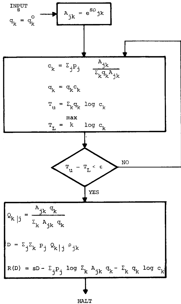
Fig. 3. Rate-distortion algorithm.
